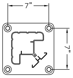
BOLT PATTERN (TYP. 9 PLACES)
