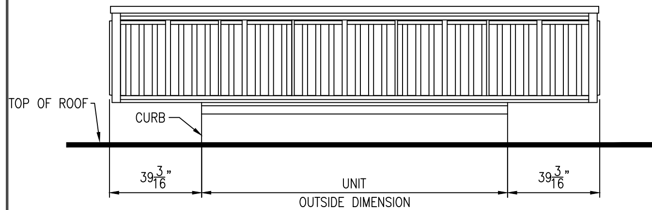
35" VERTICAL STYLE ENVISOR ELEVATION
