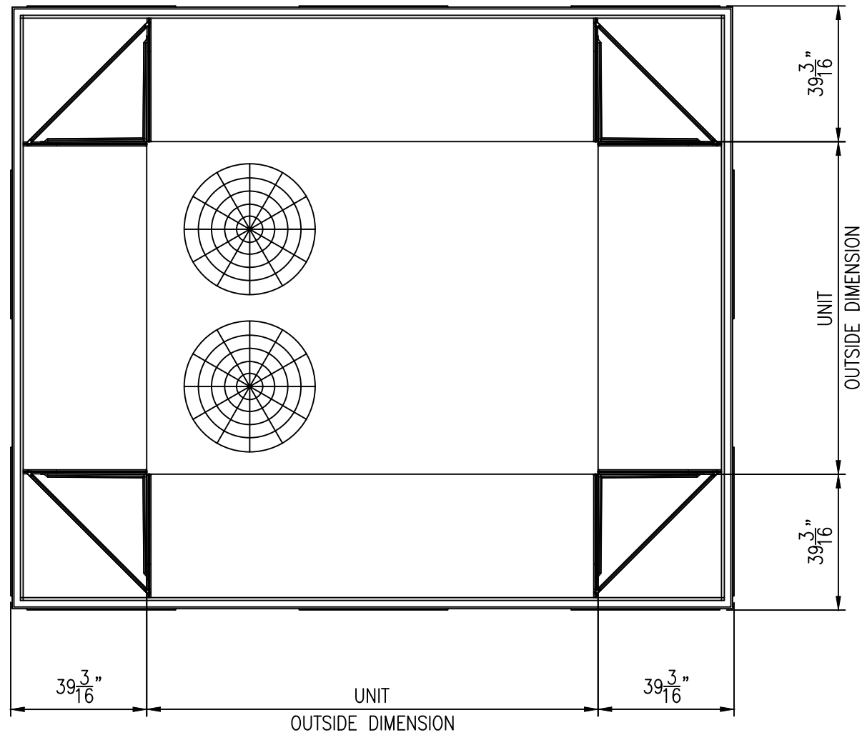
35" VERTICAL STYLE ENVISOR FOOTPRINT
