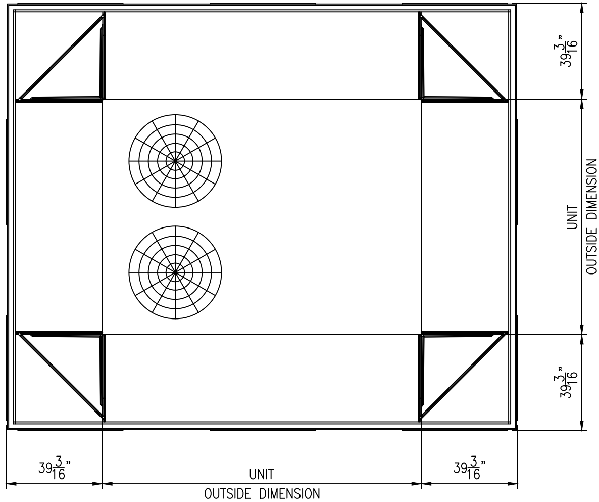
52" VERTICAL STYLE ENVISOR ELEVATION
