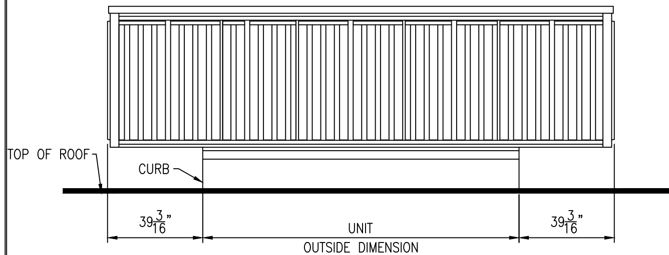
52" VERTICAL STYLE ENVISOR ELEVATION
